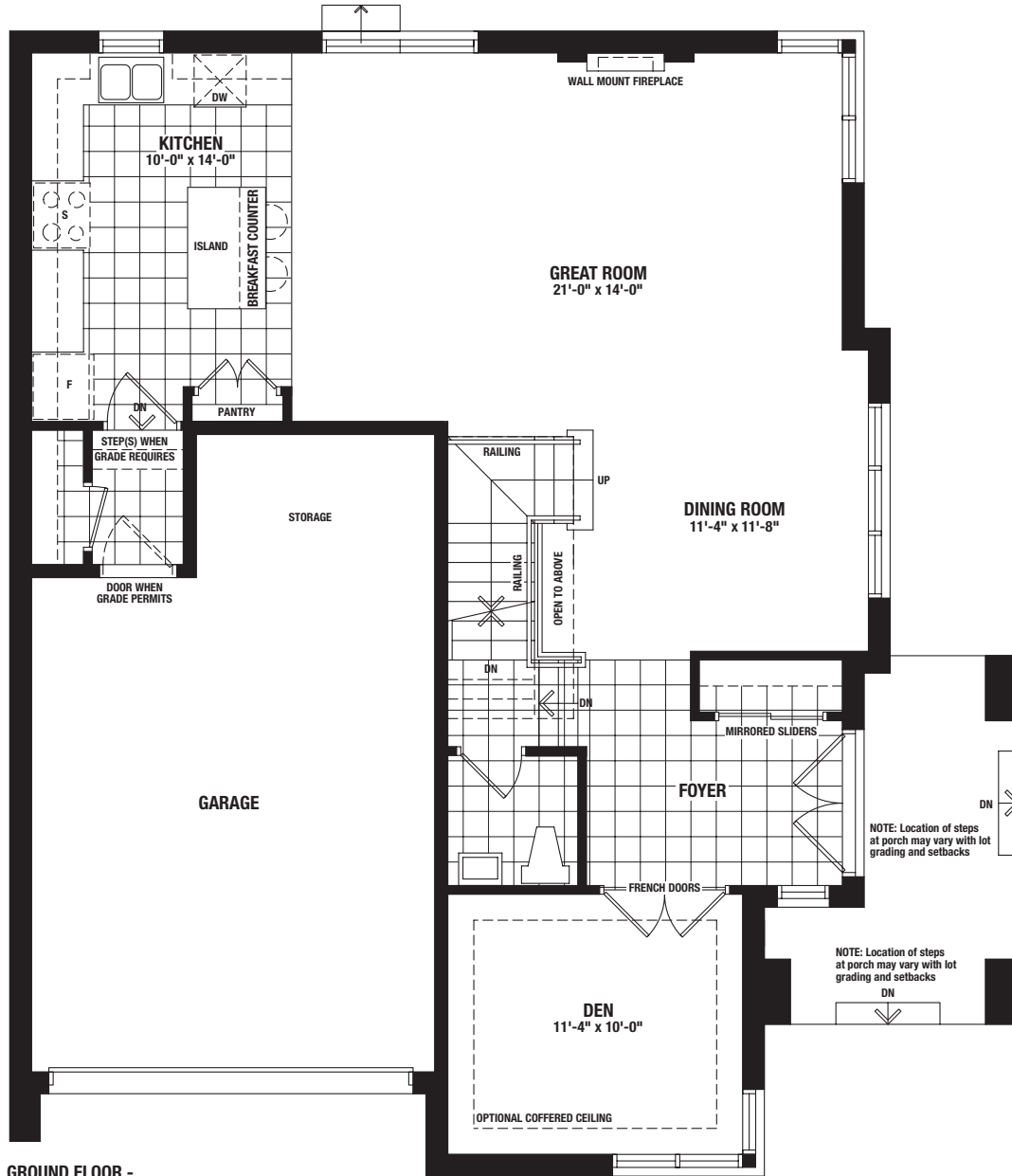
GROUND FLOOR - ELEVATION B
