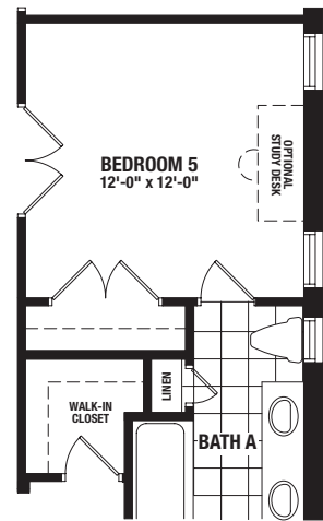
PARTIAL SECOND FLOOR - OPTIONAL BEDROOM 5 ELEVATION A/B
