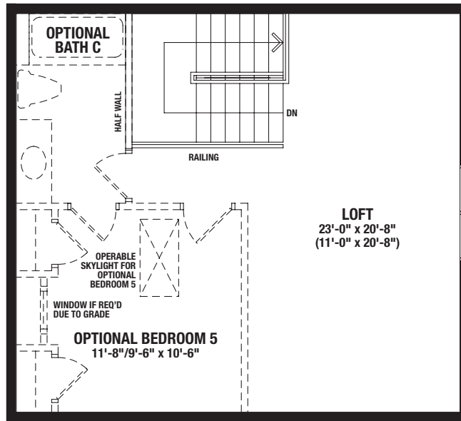
FINISHED LOFT - ELEVATION A & B
