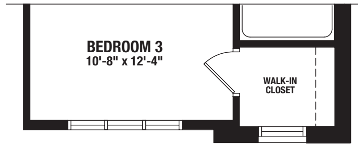
PARTIAL UPPER FLOOR - ELEVATION B
