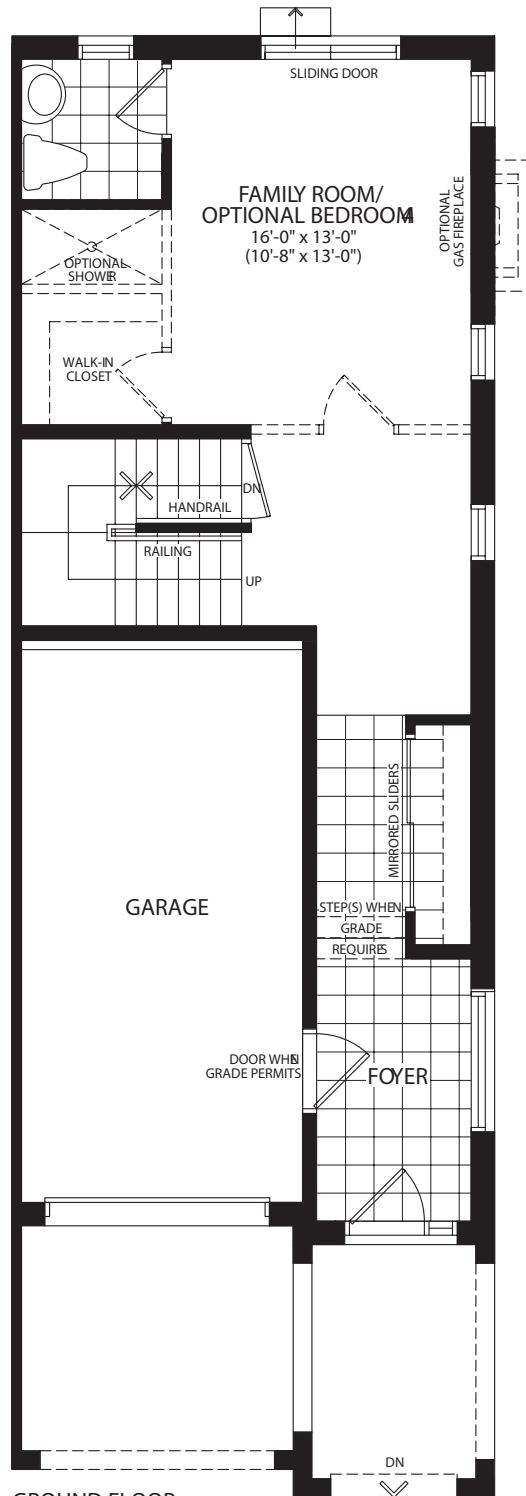
GROUND FLOOR - ELEVATION A & B
