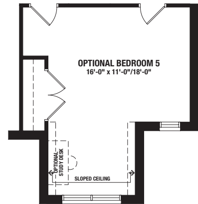
PARTIAL SECOND FLOOR - OPTIONAL BEDROOM 5 ELEVATION B
