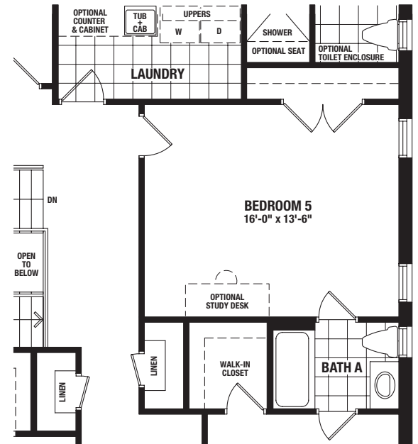
PARTIAL SECOND FLOOR - OPTIONAL BEDROOM 5 ELEVATION A/B
