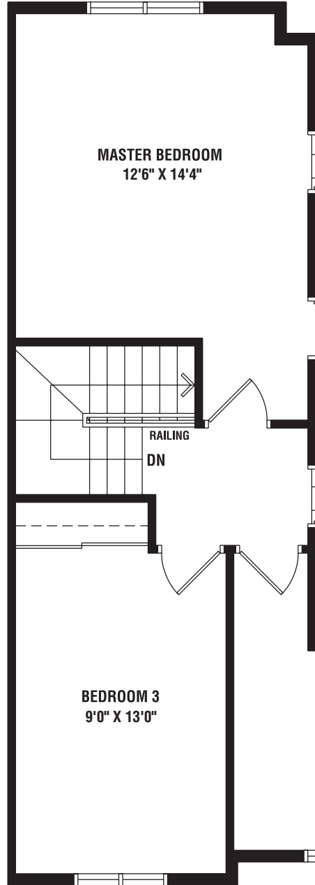
PARTIAL UPPER FLOOR ELEVATION B
