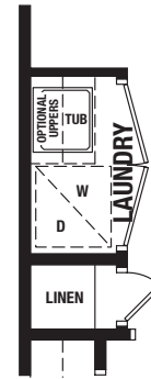
PARTIAL UPPER FLOOR OPTIONAL LAUNDRY LAYOUT - ELEVATION A & B
