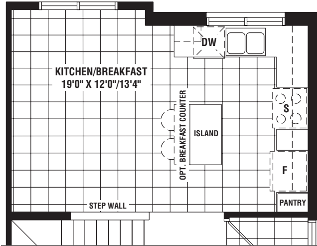
PARTIAL MAIN FLOOR ELEVATION B
