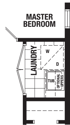
PARTIAL UPPER FLOOR OPTIONAL LAUNDRY LAYOUT - ELEVATION A & B
