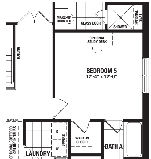
PARTIAL SECOND FLOOR - OPTIONAL BEDROOM 5 ELEVATION A/B
