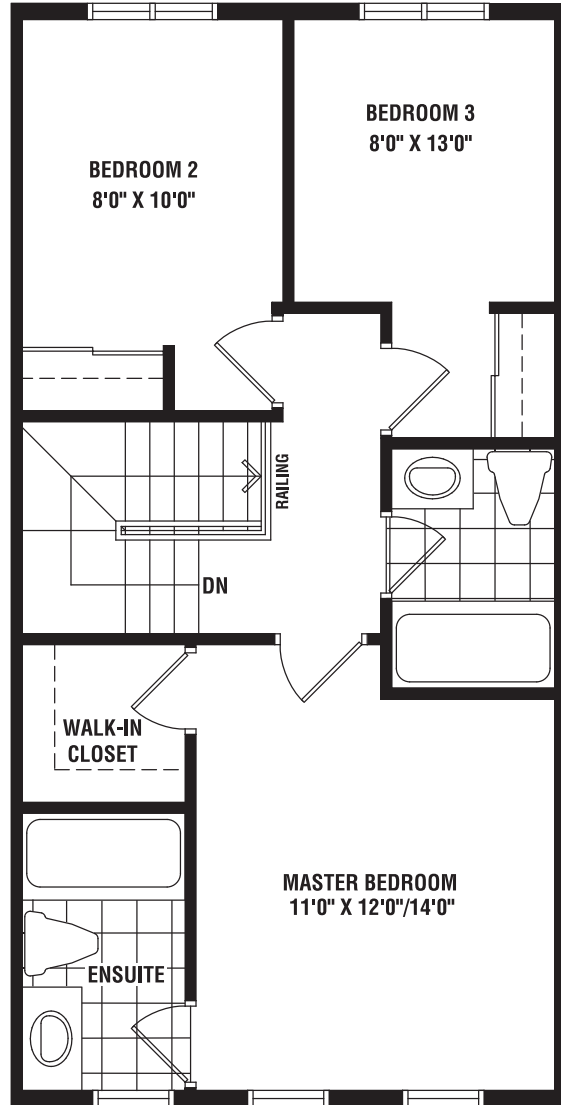
UPPER FLOOR ELEVATION A & B
