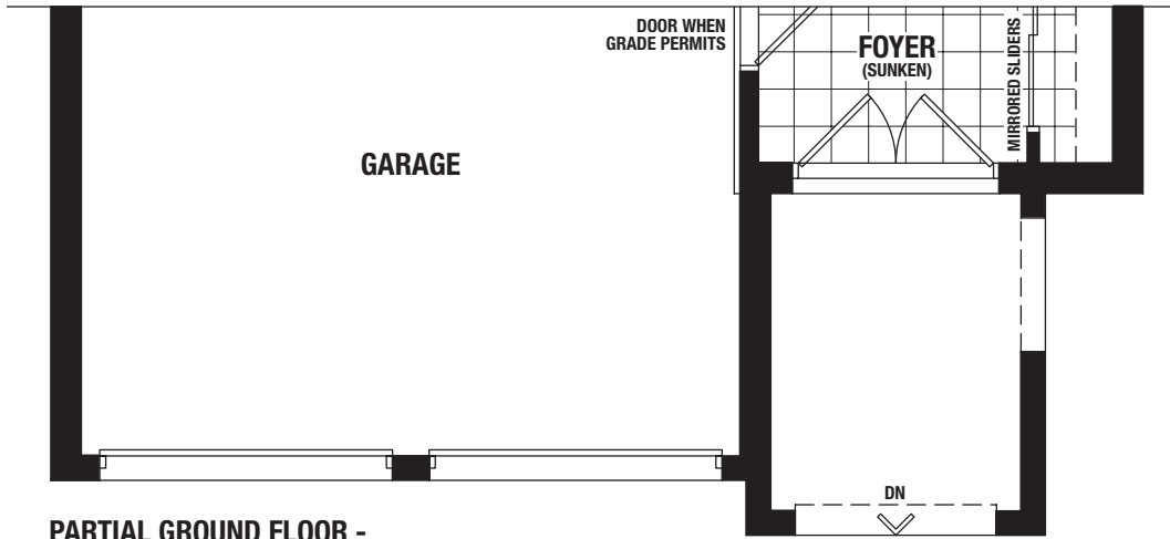
PARTIAL GROUND FLOOR - ELEVATION B
