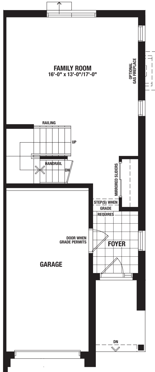
GROUND FLOOR - ELEVATION A
