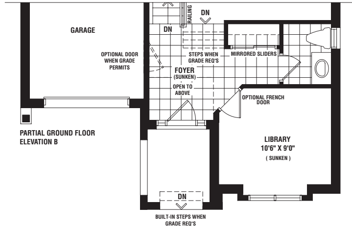
PARTIAL GROUND FLOOR ELEVATION B
