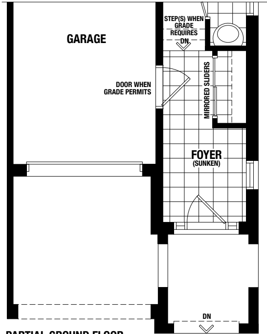
PARTIAL GROUND FLOOR - ELEVATION B
