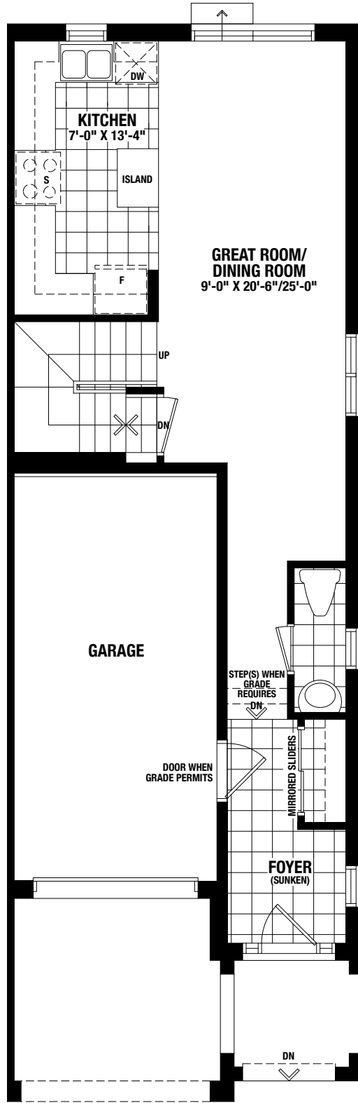
GROUND FLOOR - ELEVATION A
