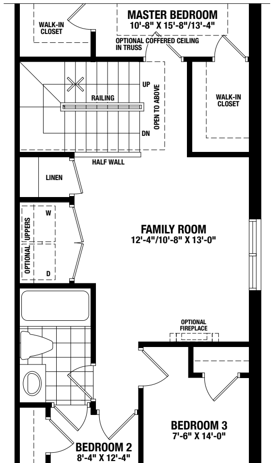
PARTIAL SECOND FLOOR OPTIONAL FAMILY ROOM LAYOUT - ELEVATION A & B
