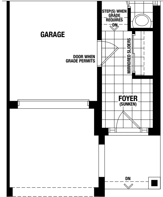
PARTIAL GROUND FLOOR - ELEVATION B
