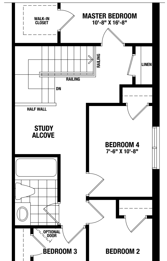
PARTIAL SECOND FLOOR OPTIONAL 4 BEDROOM LAYOUT - ELEVATION A & B
