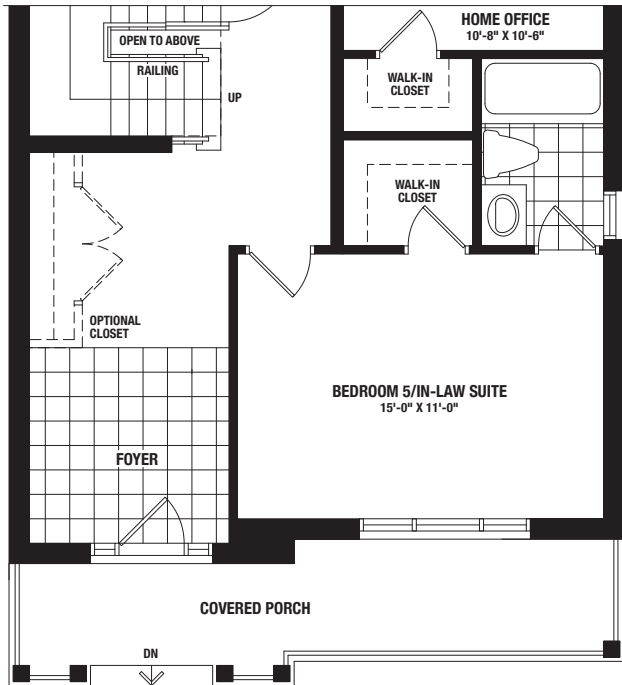
PARTIAL GROUND FLOOR - OPTIONAL BEDROOM 5/IN-LAW SUITE ELEVATION B
