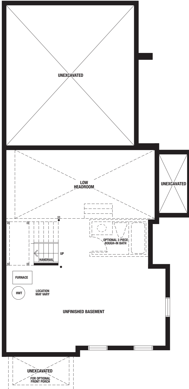
BASEMENT - ELEVATION A
