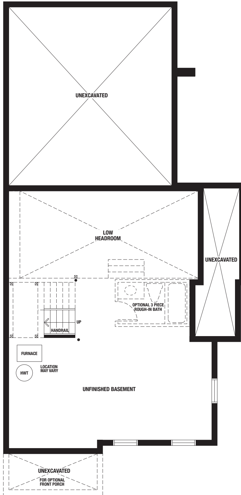
BASEMENT - ELEVATION B
