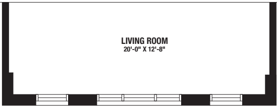
PARTIAL MAIN FLOOR - ELEVATION B
