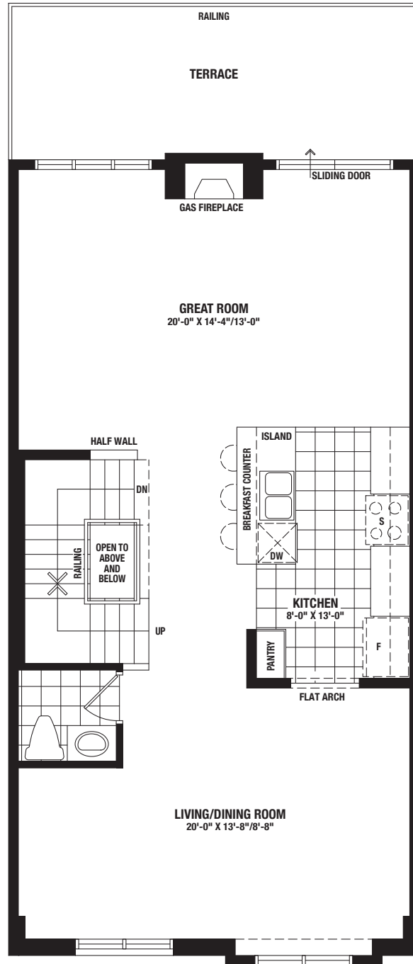
MAIN FLOOR - ELEVATION A & B
