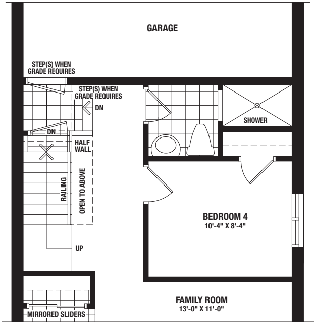
PARTIAL GROUND FLOOR - OPTIONAL BEDROOM 4 ELEVATION A & B
