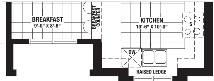
PARTIAL MAIN FLOOR - ELEVATION B
