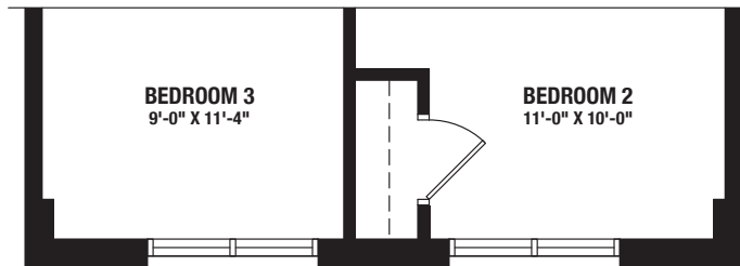
PARTIAL UPPER FLOOR - ELEVATION B
