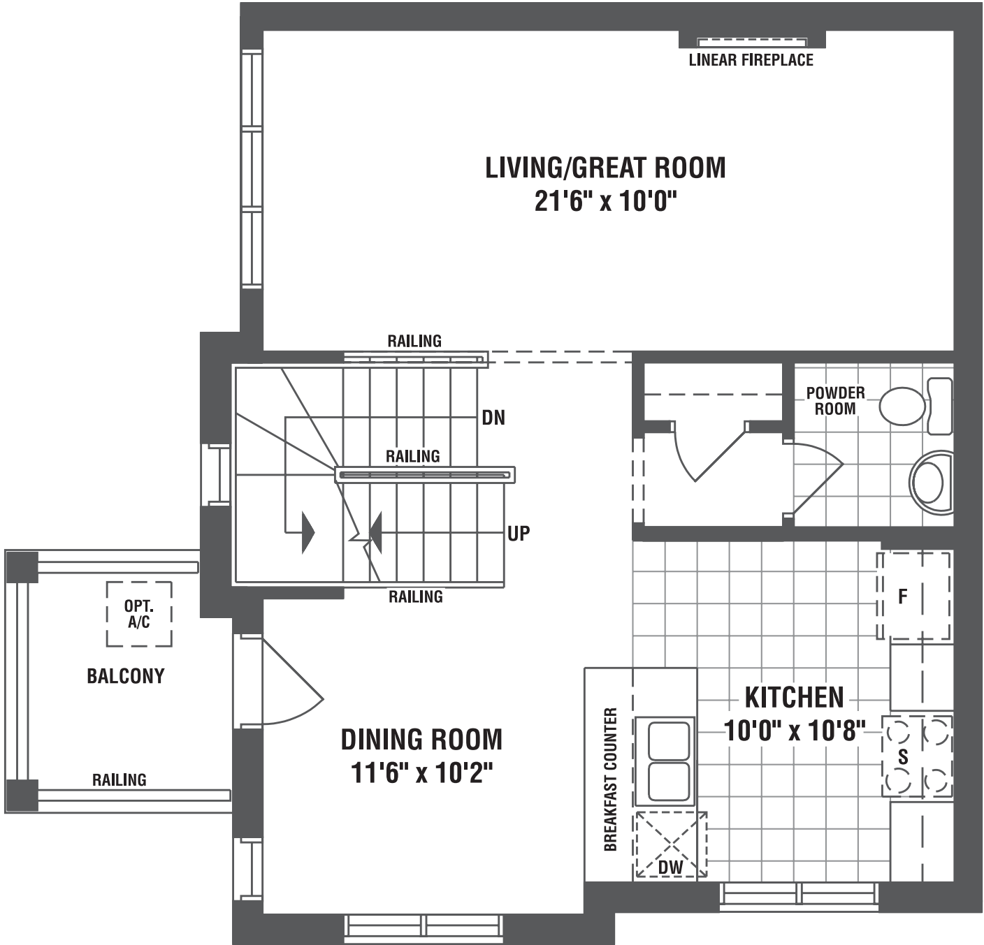
MAIN FLOOR ELEVATION A
