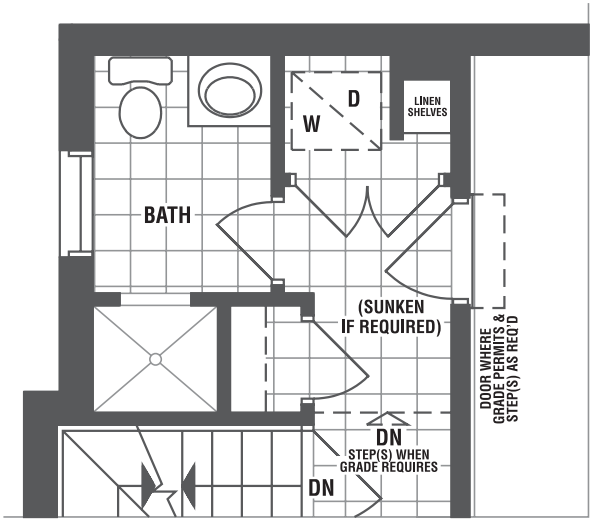
PARTIAL GROUND FLOOR OPTIONAL FULL BATHROOM ELEVATION A
