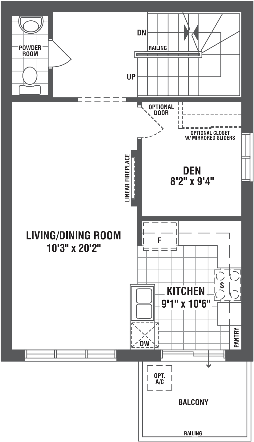
MAIN FLOOR ELEVATION AE/BE
