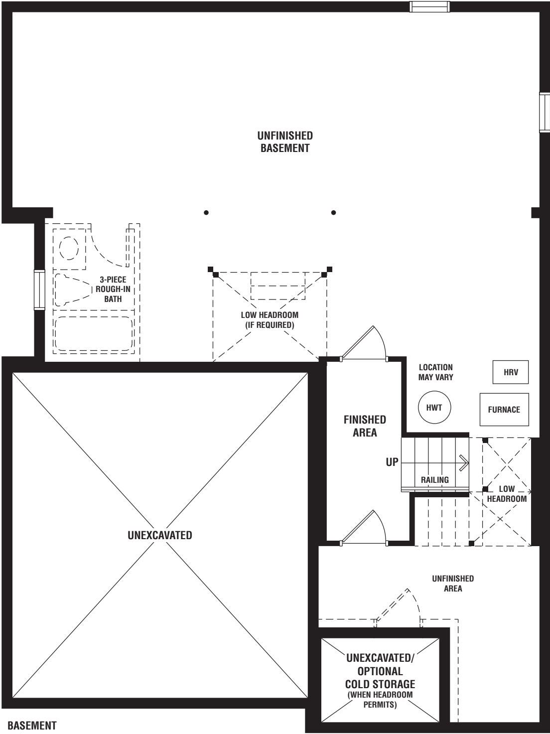
BASEMENT ELEVATION A
