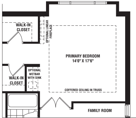
PARTIAL SECOND FLOOR OPTIONAL PRIMARY BEDROOM WITH WET BAR ELEVATION A & B
