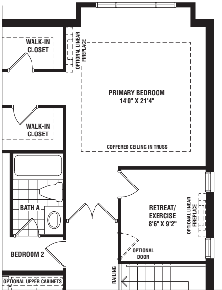
PARTIAL SECOND FLOOR OPTIONAL PRIMARY BEDROOM WITH RETREAT / EXERCISE ROOM ELEVATION A & B
